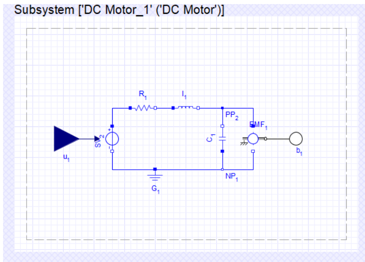
Figure 2.12: DC Motor Subsystem
