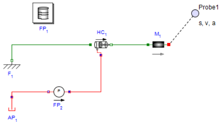
Figure 6.18: Translational Motion with Fixed Pressure Source
