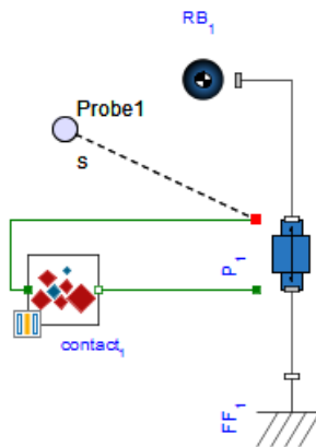
Figure 6.7: Bouncing Ball
