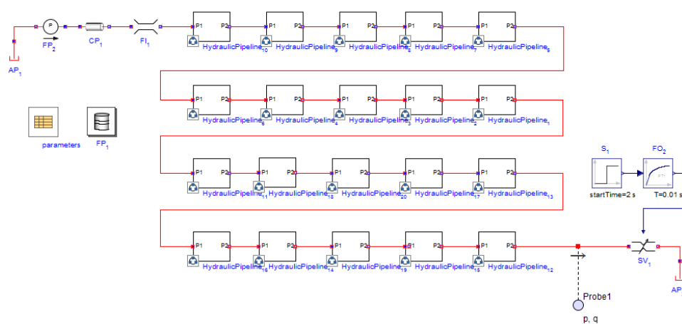
Figure 6.27: Water Hammer
