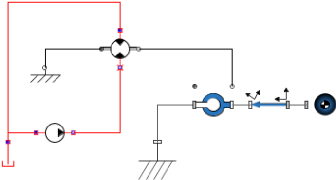
Figure 6.21: Rotational Fixed Flange Hydraulic component
